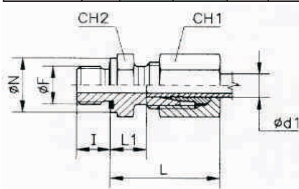
Adaptor drept TN92-SR*
