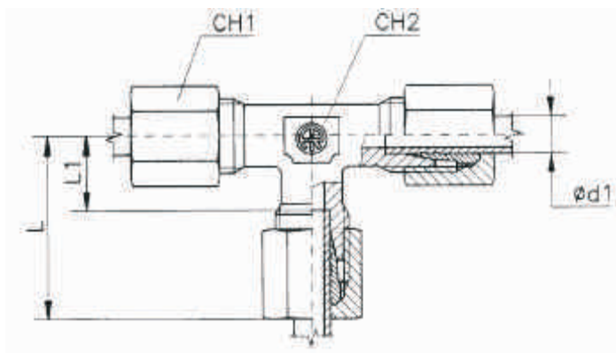
Adaptor T TN100*
