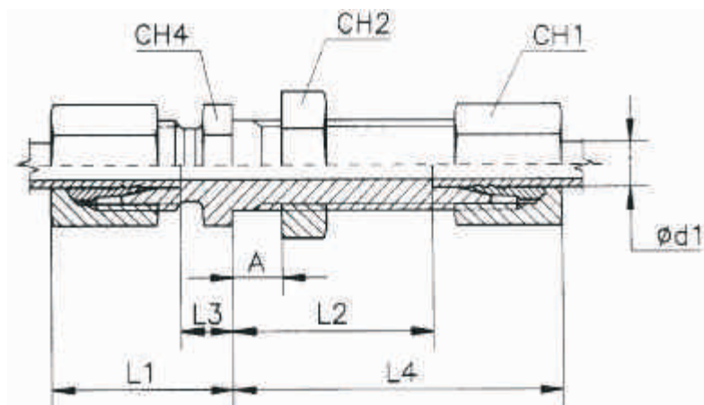
Adaptor drept TN102*
