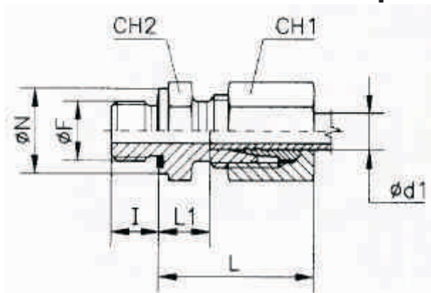
Adaptor drept TN92-SM*
