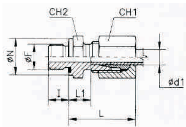
Adaptor drept TN92-LR*
